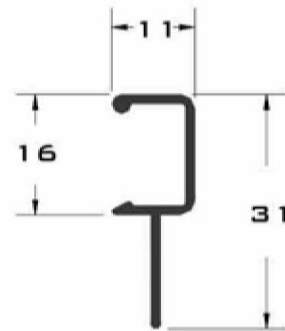
3534 GUIA MOSQUITERO
