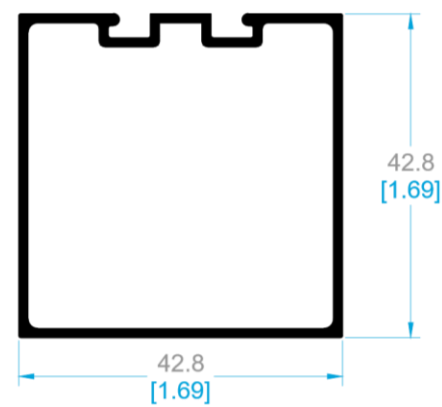
9184 REMATE.
